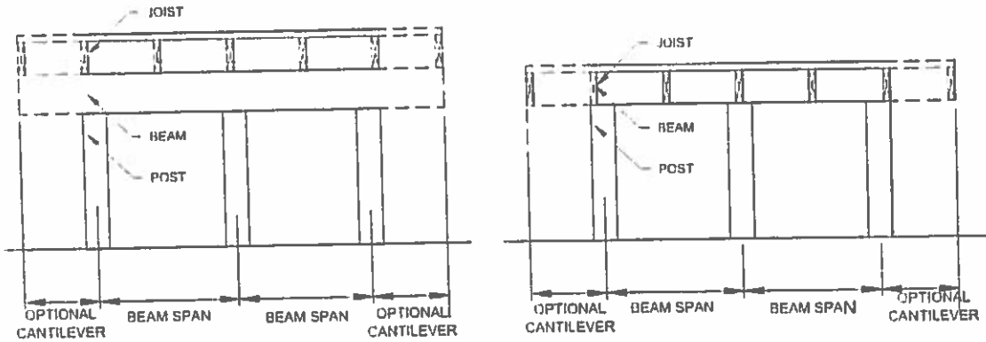
FLUSH BEAM
